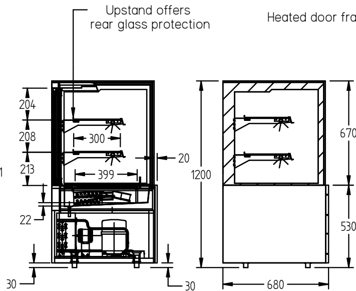
Section View
