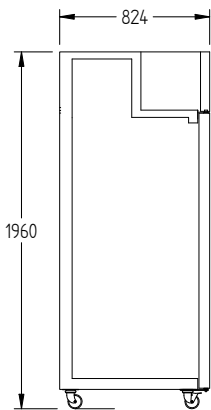
J1SA MODEL J2SA MODEL SIDE VIEW
