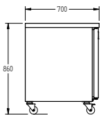
TU2SDSS/TU3DSS MODEL SIDE VIEW
