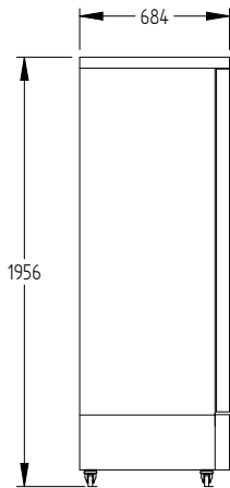
J400 MODEL SIDE VIEW
