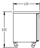
TU2SDSS-12 MODEL SIDE VIEW
